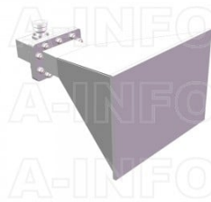
LB-284-15-C-7/16FSPO Standard Gain Horn Antenna 2.6-3.95GHz 15dB Gain 7/16(DIN) Female
